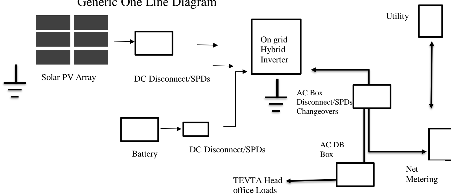
Generic One Line Diagram
